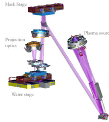
Schematic of Extreme Ultra Violet Lithography. Source: Sweeney, D. (1999): Extreme Ultraviolet Lithography: Imaging the Future. In: Science & Technology Review, 11: 6.
